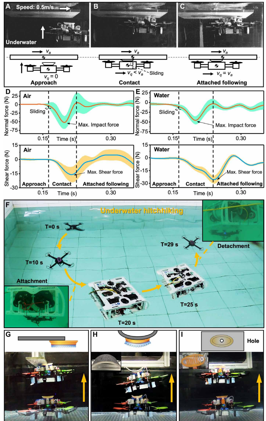
Fig. 6. Hitchhiking onto a moving object and adhesive performance of the aerial-aquatic robot. (A to C) High-speed images of the robot hitchhiking onto a moving plate (smooth acrylic) under water. The plate moves from the left to the right at controlled speeds. The robot moves vertically upward until it attaches to the plate. The hitchhiking process was divided into three stages. A video of hitchhiking onto the moving surface is available in movie S13. (A) The approach stage, (B) the contact stage, and (C) the attached-following stage. Note that the high-speed camera was mounted on the moving carriage and has the same speed and direction as the plate. The plate's vertical and shear forces were measured as the robot hitchhiked through the air (D) and under water (E) as the plate moved at a speed of 0.5 m/s ( N=3 ). Shaded error bars represent \pm 1 SD. Curves were fitted by B-splines. (F) The robot demonstrating hitchhiking behavior in a laboratory pool (see movie S13). The inset images were taken underwater and showed the robot's attachment and detachment to the host (a remotely operated vehicle). (G to I) Demonstrating the robot's redundant adhesion ability. (G) The robot can attach to the narrow acrylic surface with only half of its disc. (H) The robot can also adhere to a curved, rough surface and a damaged surface with a 10 mm-diameter hole in the middle (I).
