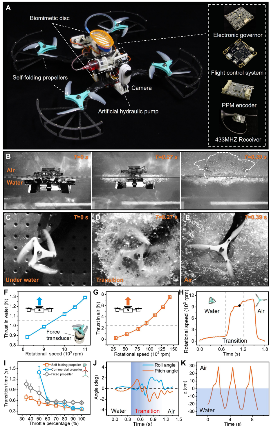
Fig. 5. Aerial-aquatic hitchhiking robot with self-folding propellers and its air/water transition performance. This robot is self-contained; it can be remotely controlled for flying, swimming, and attaching to surfaces in air and water, and it transits across the two media. (A) Top view of the untethered robot and its main components. (B) Images of the robot taking off from water at various time instants in a laboratory water tank. (C to E) Self-folding propeller performance during the water-to-air transition. (C) The propeller remains folded underwater while rotating. (D) High-speed image of the propeller extending on its own at the water-air interface. (E) The propeller fully unfolds in the air. (F and G) Thrust force of the self-folded propeller at different rotational speeds under water (F) and in the air (G) ( N=5 ). The critical rotational speeds (and corresponding forces) are marked by dashed horizontal lines in (F) and (G). By exceeding the critical rotational speeds (actuated by the same throttle percentage of motor), the robot can move upward underwater [blue dashed line in (F)] or fly up in air [red dashed line in (G)]. (H) The propeller's rotational speed (averaged across all four rotors) as a function of time during the transition from water to air. The area between the two black dashed lines represents the transition process, which started from when the robot's propellers touched the water surface and ended when the robot was entirely out of the water. The black dot indicates when the self-folding propeller achieved the necessary rotational speed to lift the robot up (8500 rpm). (I) Comparison of the transition time of the self-folding propeller, commercial propeller, and self-folding propeller fixed in an unfolded state across different throttle percentages ( N=5 ). (J) The roll and pitch angles of the robot versus time during one typical water-to-air transition. (K) Three typical cycles of the robot continuously transiting the air-water boundary (movie S10). All error bars represent \pm 1 SD.
